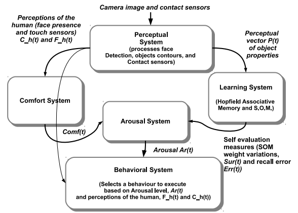
Figure 1: Components of the robot architecture used in the experiments. The Perceptual System processes the perception into a binary perceptual vector to be learned by the Learning System. We then evaluate the Stimulation as in Eq. 1, which is used with the comfort (Eq. 3) to compute the Arousal level in Eq. 2. The arousal level is used by the Behavioral System to choose the action to be performed.
